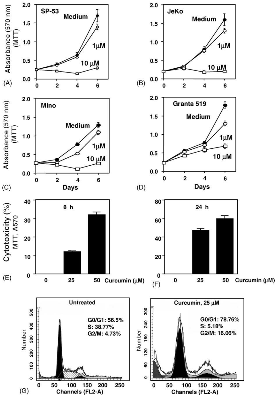
Fig. 4. Curcumin inhibits proliferation in MCL cells. (A) SP-53; (B) JeKo-1; (C) Mino; or (D) Granta 519 (5000 cells/0.1 ml) were incubated at 37 °C with curcumin (1 and 10 \mu M) for indicated time duration, and the viable cells were assayed using MTT reagent. The results are shown as the mean \pm S.D. from triplicate cultures. (E, F) SP-53 cells (5000/0.1 ml) were incubated at 37 °C with curcumin (25 and 50 \mu M) for 8 and 24 h, and then cell viability determined using MTT method. The results are shown as the mean \pm S.D. of triplicates. (G) Curcumin arrests the cells at G1/S phase of the cell cycle. Serum-starved SP-53 cells ( 2 \times 10^6 cells/ml) were incubated in the absence or in presence of different doses of curcumin for 36 h. Thereafter, the cells were washed, fixed, stained with propidium iodide, and analyzed for DNA content by flow cytometry as described in Section 2.
