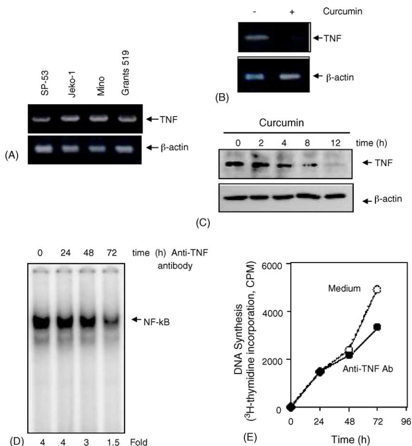
Fig. 7. TNF is an autocrine growth factor for MCL. (A) MCL express TNF mRNA. Two million cells/ml were tested for TNF by RT-PCR. \beta -actin was used as a loading control. (B) Curcumin inhibits expression of TNF mRNA. Five million Granta 519 cells were treated with curcumin (50 \mu M) for 3 h, and tested for TNF by RT-PCR. (C) Curcumin inhibits expression of TNF protein. Two million SP-53 cells were treated with curcumin (50 \mu M) for indicated time points, and tested for TNF by Western blot. (D) Anti-TNF antibody inhibits constitutive NF- \kappa B activation. Two million SP-53 cells were treated with anti-TNF antibody (50 ng/ml) for indicated times, then nuclear extract was prepared and examined for NF- \kappa B. (E) Anti-TNF antibody inhibits proliferation of MCL cells. SP-53 cells (5000/0.1 ml) were incubated at 37 ^{\circ} C with anti-TNF antibody (50 ng/ml) for indicated time points, and then cell proliferation was determined using ^3 H-thymidine incorporation. The results are shown as the mean \pm S.D. of triplicates.
