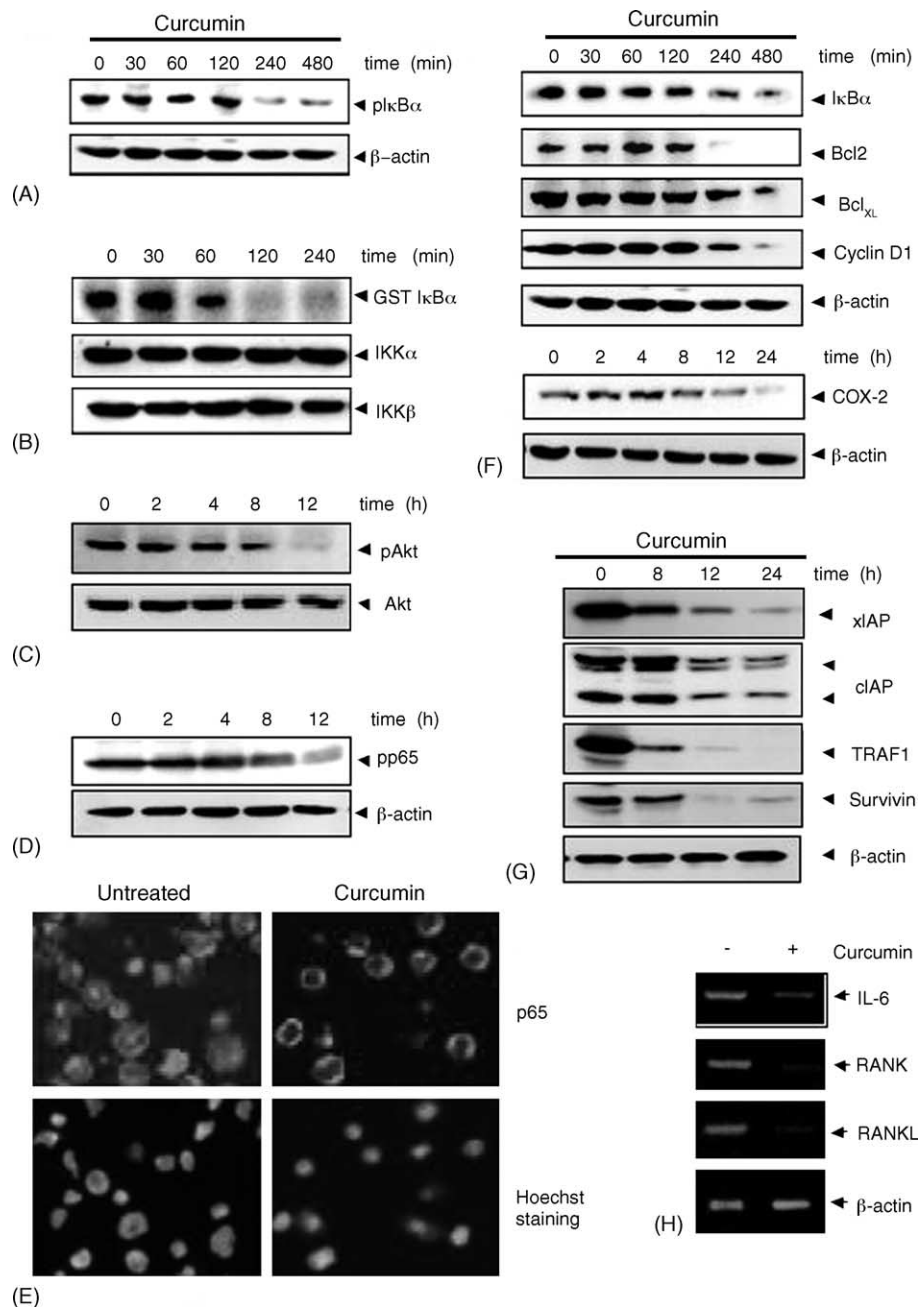
Fig. 3. Curcumin inhibits IκBα phosphorylation, IκB kinase, p65-phosphorylation, and induces redistribution of p65. (A) Two million SP-53 MCL cells were treated with curcumin (50 μM) for indicated times, and cytoplasmic extracts were prepared and examined for the level of phosphorylated IκBα by Western blotting. (B) Five million SP-53 MCL cells were treated with curcumin (50 μM) for indicated times, and whole-cell extracts were prepared and immunoprecipitated with IKK antibodies and examined by the immunocomplex kinase assay for IKK activity (upper panel) or by Western blotting for total IKKα and IKKβ proteins (middle and lower panel). (C) Two million SP-53 MCL cells were treated with curcumin (50 μM) for indicated times, and whole-cell extracts were prepared and examined for the level of phosphorylated Akt by Western blotting. (D) Two million SP-53 MCL cells were treated with curcumin (50 μM) for indicated times, and cytoplasmic extracts were prepared and examined for the level of phosphorylated p65 by Western blotting. (E) SP-53 cells were incubated with or without curcumin (50 μM) for 3 h and then analyzed for the distribution of p65 by immunocytochemistry. Red stain indicates the localization of p65, and blue stain indicates the nucleus (magnification, 200×). Curcumin inhibits NF-κB-regulated gene products. (F) Two million SP-53 cells were treated with curcumin (50 μM) for indicated times, and cytoplasmic extracts were prepared. Sixty micrograms of cytoplasmic extracts were resolved on 10% SDS-PAGE gel, electrotransferred onto a nitrocellulose membrane, and probed for IκBα; Bcl-2, Bcl-xL, cyclin D1, and COX-2. The same blots were stripped and reprobed with anti-β-actin antibody to show equal protein loading (lower panel in each figure). (G) Two million SP-53 cells were treated with curcumin (50 μM) for indicated times, and whole-cell extracts were prepared. Fifty micrograms of cytoplasmic extracts were resolved on 10% SDS-PAGE gel, electrotransferred onto a nitrocellulose membrane, and probed for xIAP, cIAP, TRAF1 and survivin. Same blots were stripped and reprobed with anti-β-actin antibody to show equal protein loading (lower panel in each figure). (H) Five million Granta 519 cells were treated with curcumin (50 μM) for 3 h, and total mRNA was extracted and examined for expression of IL-6, RANK, and RANKL mRNA by RT-PCR. β-actin mRNA was used as an internal control to show equal RNA loading.
